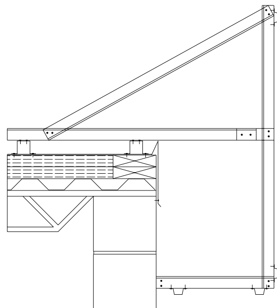
Vertical Mansard
