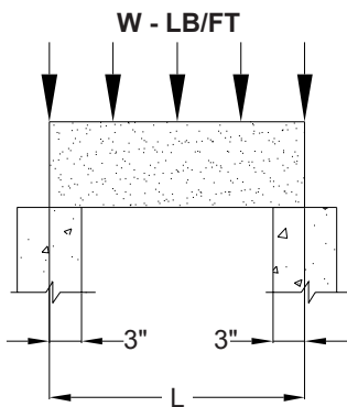
SIMPLE SPAN
