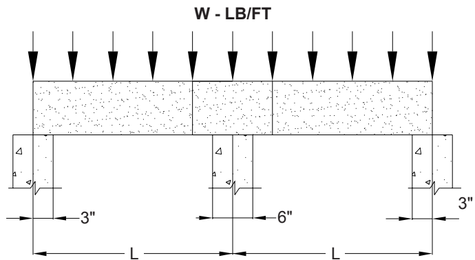
TWO SPAN
