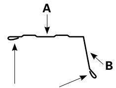
1/8" Closed Hem
